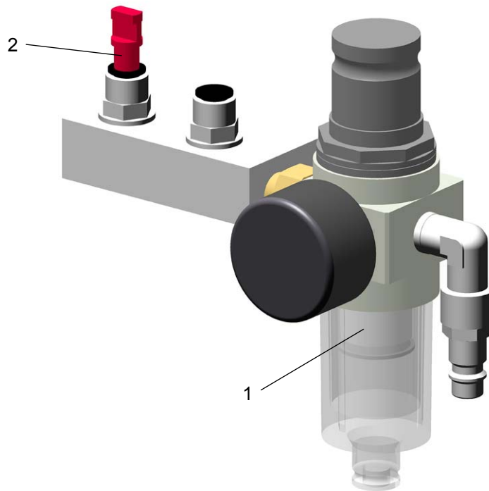
OptiFlex 2 K – Pneumatic group
